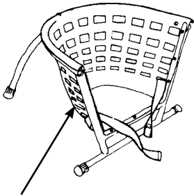
A bath seat made from half a plastic bucket or laundry basket on a tube frame:
