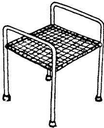
A stool with a seat woven from strips of car tire inner tube:
